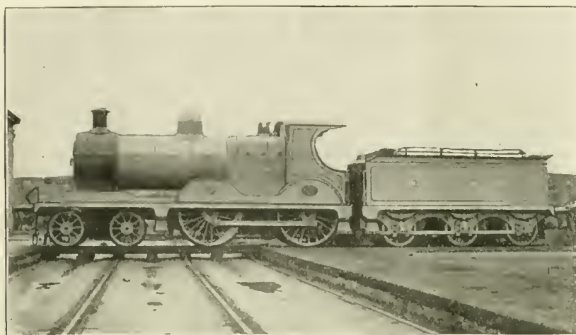
IRISH EIGHT-WHEEL ENGINE.—M. G. W. R.
